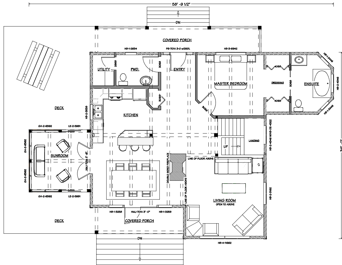
MAIN FLOOR PLAN 1404 SQ.FT
