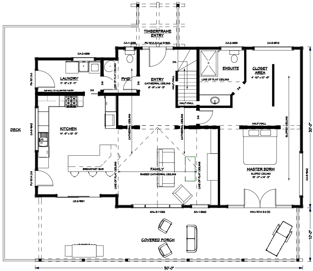
MAIN FLOOR PLAN 1396 SQ.FT
