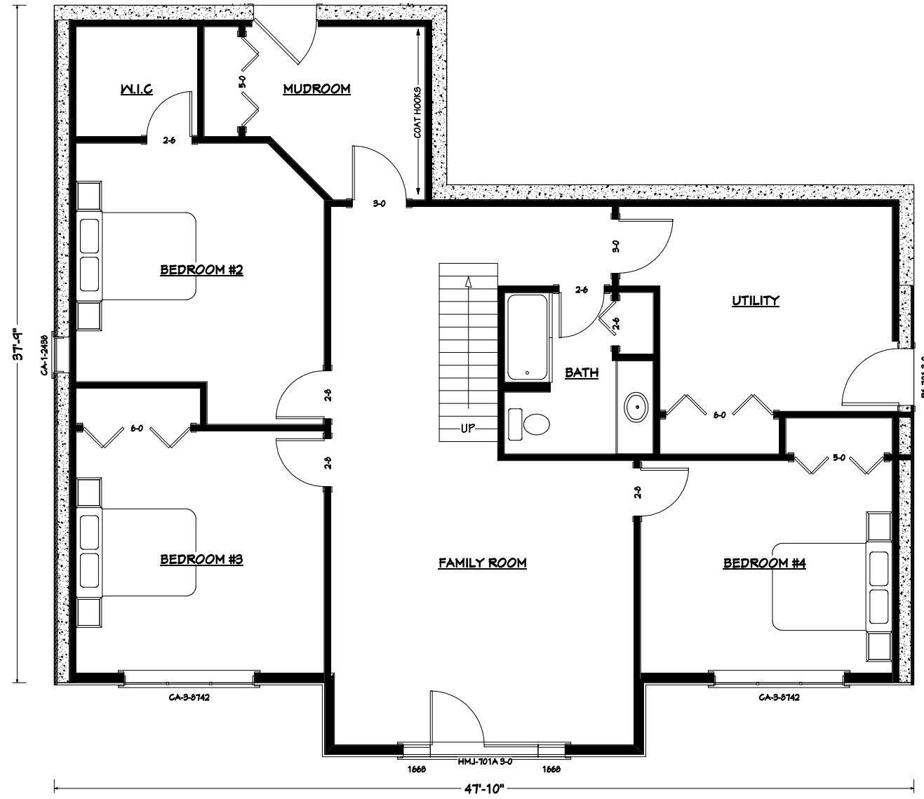
LOWER FLOOR PLAN 2000 SQ.FT
