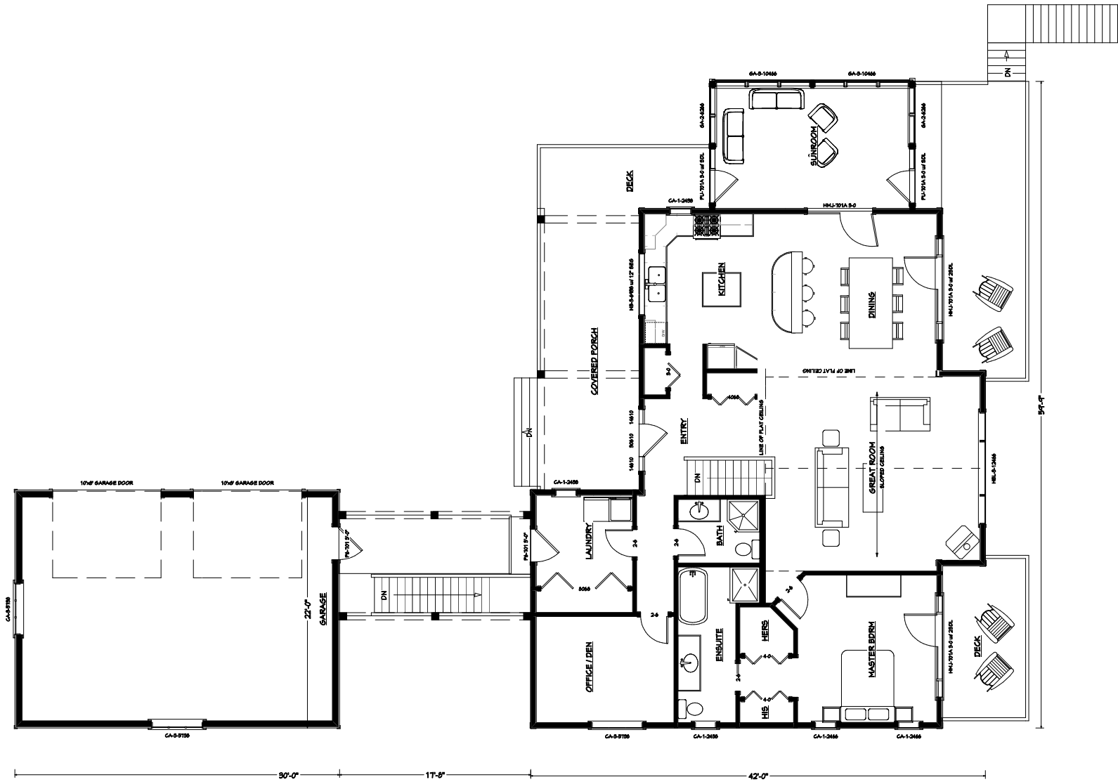
MAIN FLOOR PLAN 2195 SQ.FT
