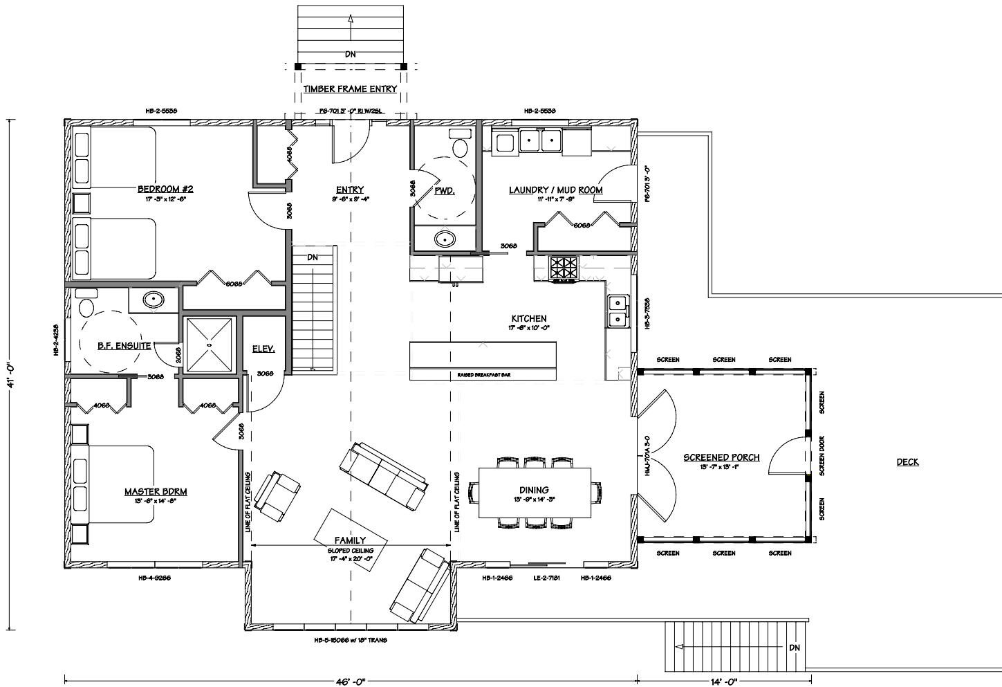
MAIN FLOOR PLAN 1741 SQ.FT
