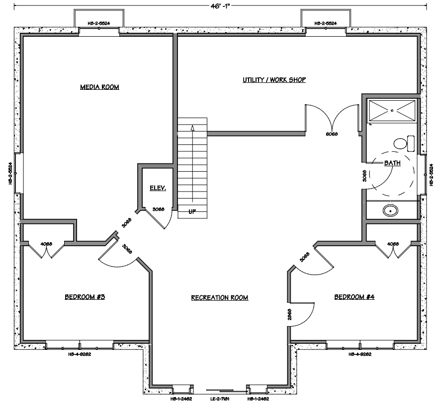
LOWER LEVEL PLAN 1741 SQ.FT
