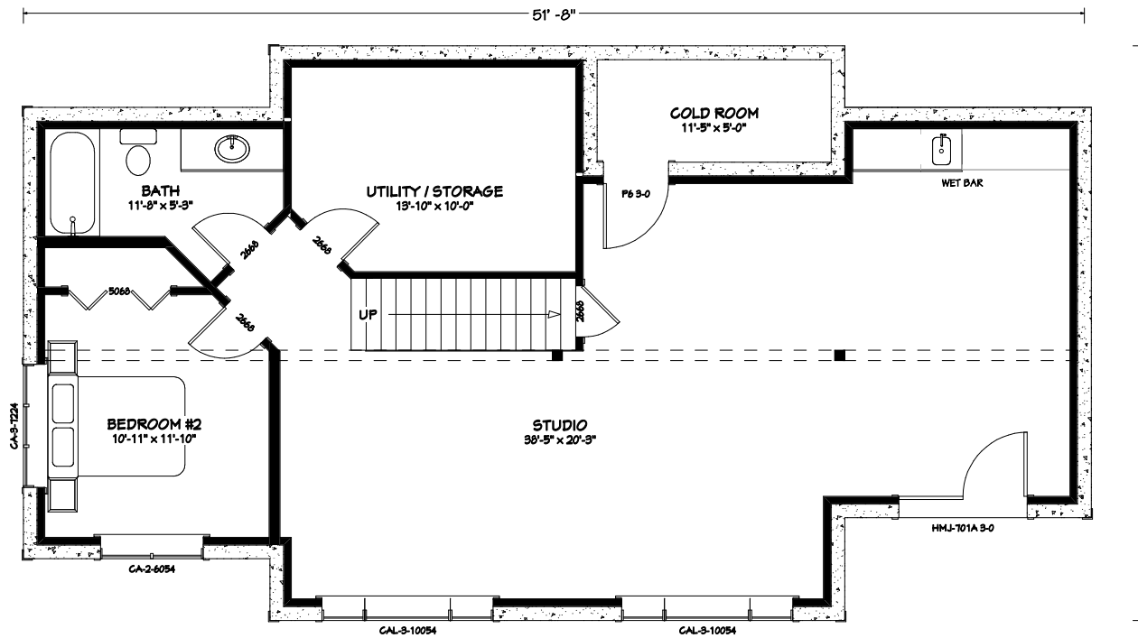
UPPER FLOOR PLAN 1227 SQ.FT
