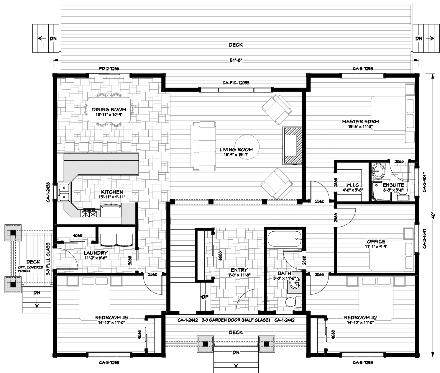
MAIN FLOOR PLAN 1906 SQ FT
