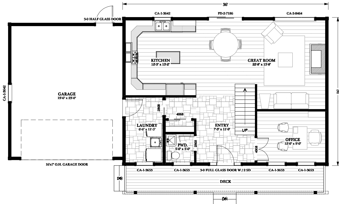
MAIN FLOOR PLAN 936 SQ FT
