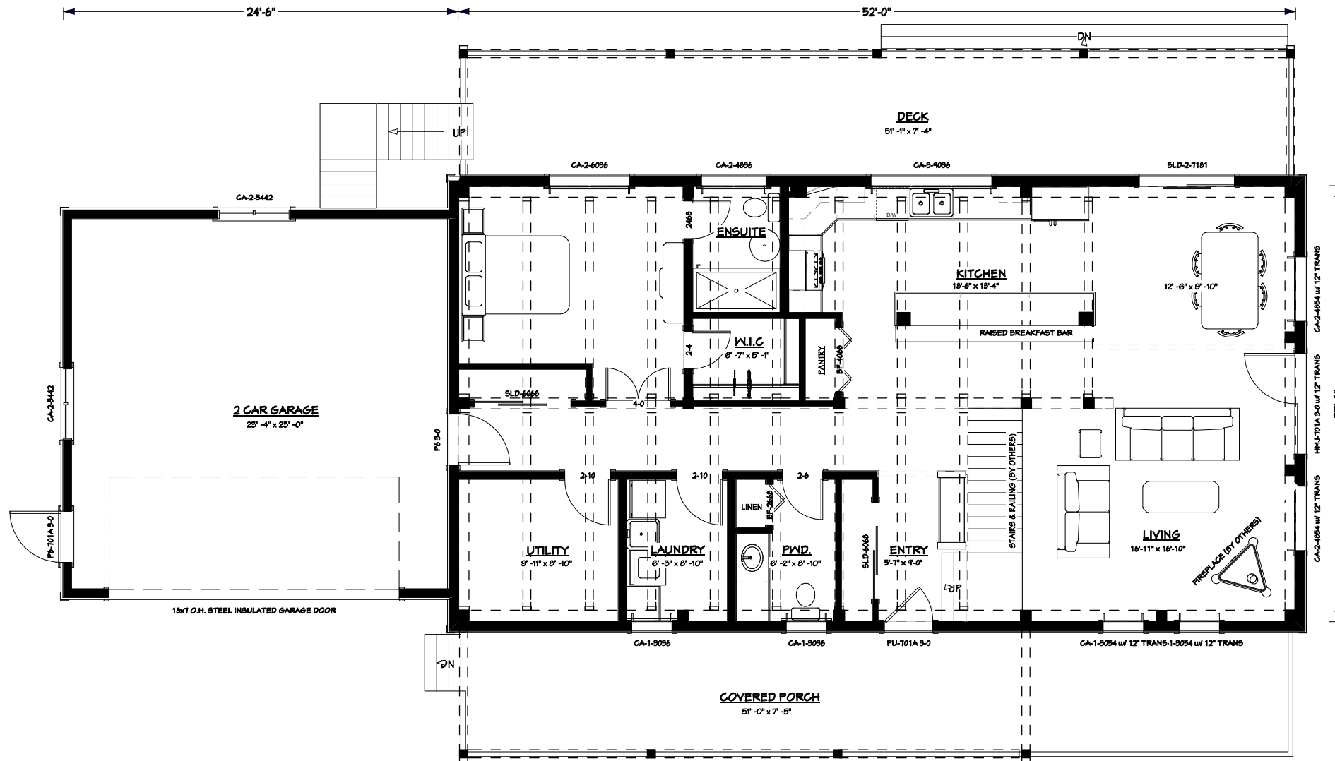
MAIN FLOOR PLAN 1242 SQ.FT
