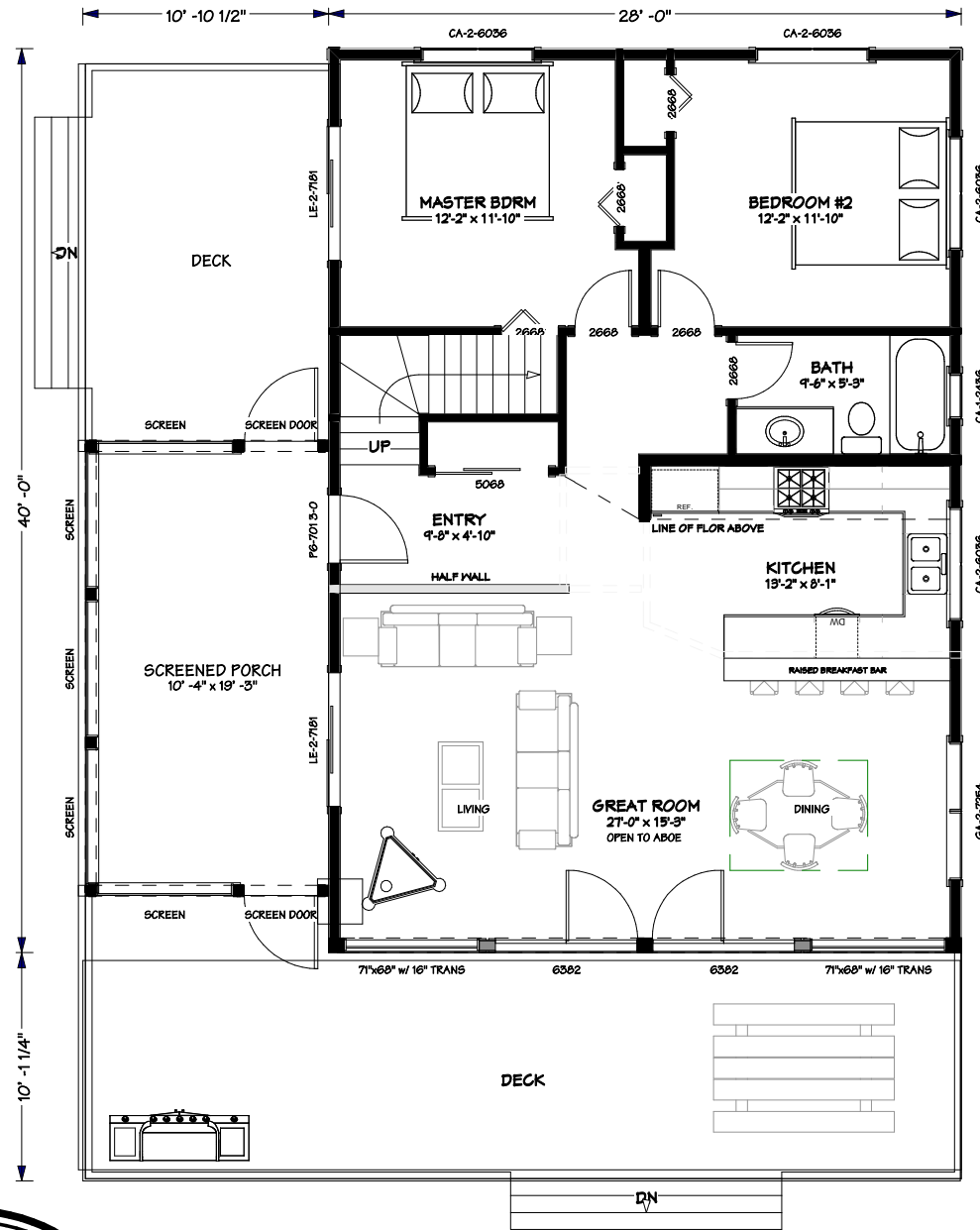
MAIN FLOOR PLAN 1117 SQ.FT
