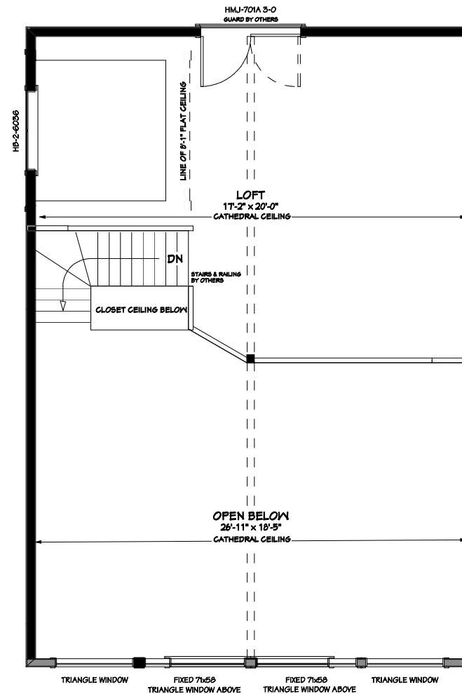
UPPER FLOOR PLAN 493 SQ.FT
